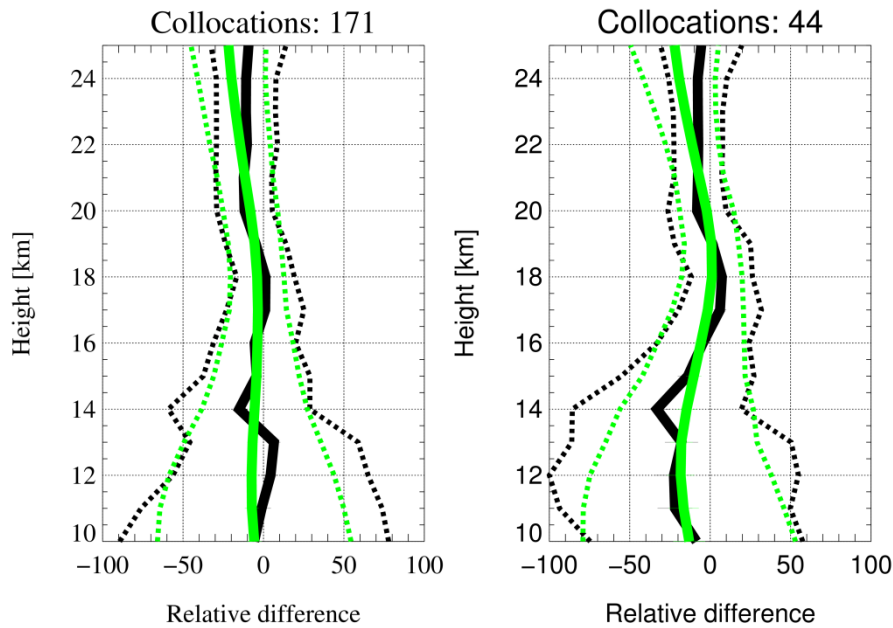
Figure 26: Comparison for SCIAMACHY V3.01 and balloon-borne CFH. Left: all possible collocations, right: collocations to the processed data set (every 8 th day globally, every 2 nd day between 45°S and 45°N). Black solid lines show the mean percentage difference for CFH data interpolated on the SCIAMACHY retrieval grid, black dotted lines the corresponding standard deviation of the bias corrected difference. Green lines show the mean percentage difference for CFH data smoothed with the SCIAMACHY AVK (solid) and the corresponding standard deviation of the bias corrected difference (dotted). In the right panel the standard error of the mean is indicated as error bars, in the left panel it is smaller than the width of the line and hence not visible.
