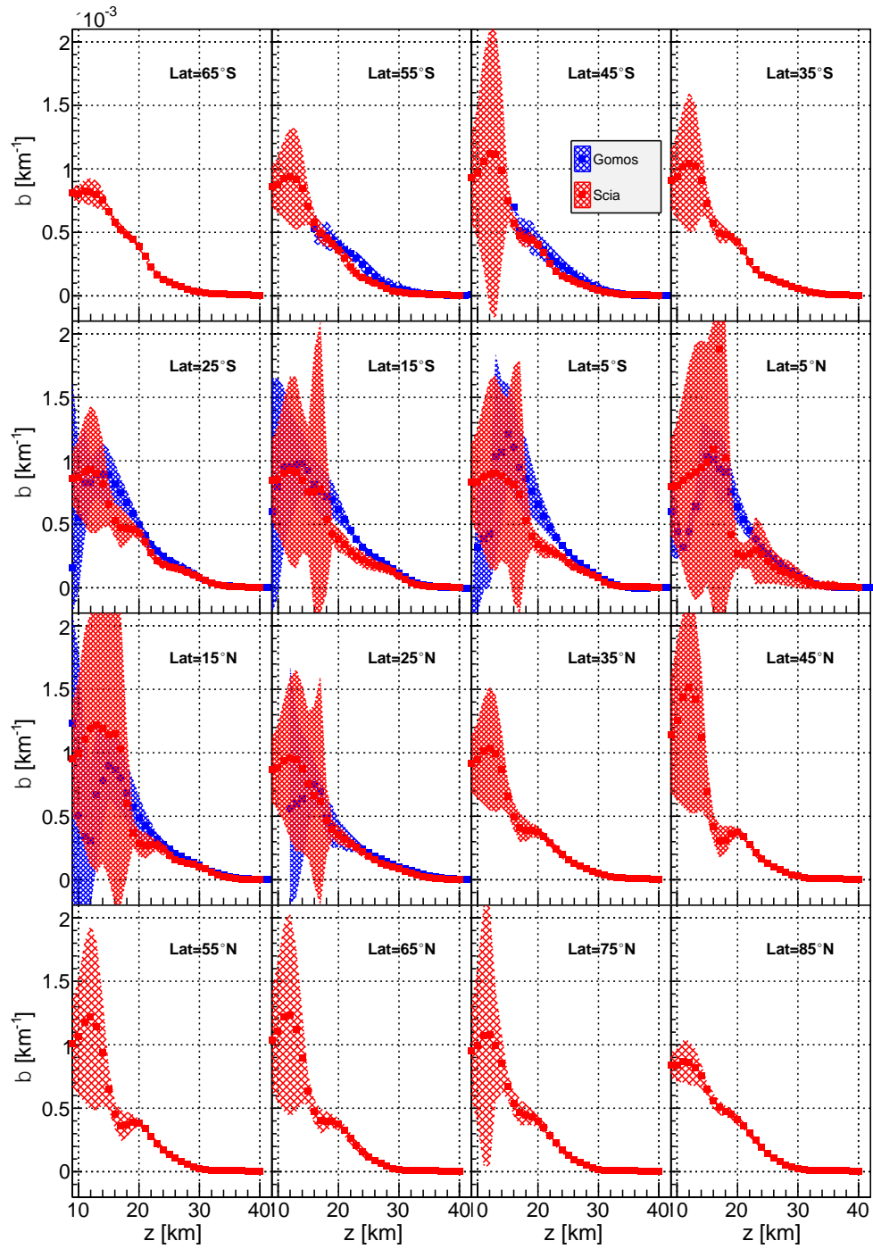
Figure 37: Monthly zonal mean aerosol extinction profiles at 470 nm from SCIAMACHY and GOMOS for June 2003.
