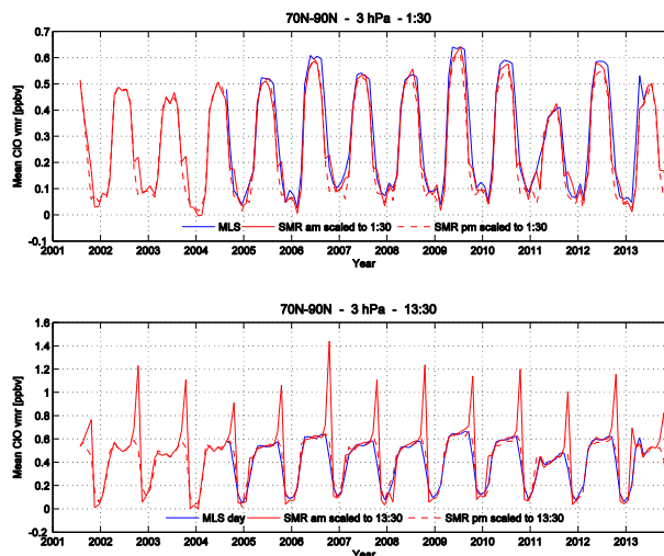
Figure 55: Comparison of scaled SMR (red) and unscaled MLS (blue) CIO time-series for the 3hPa level and northern high latitudes. Top: night (1:30am). Bottom: day (1:30pm).
