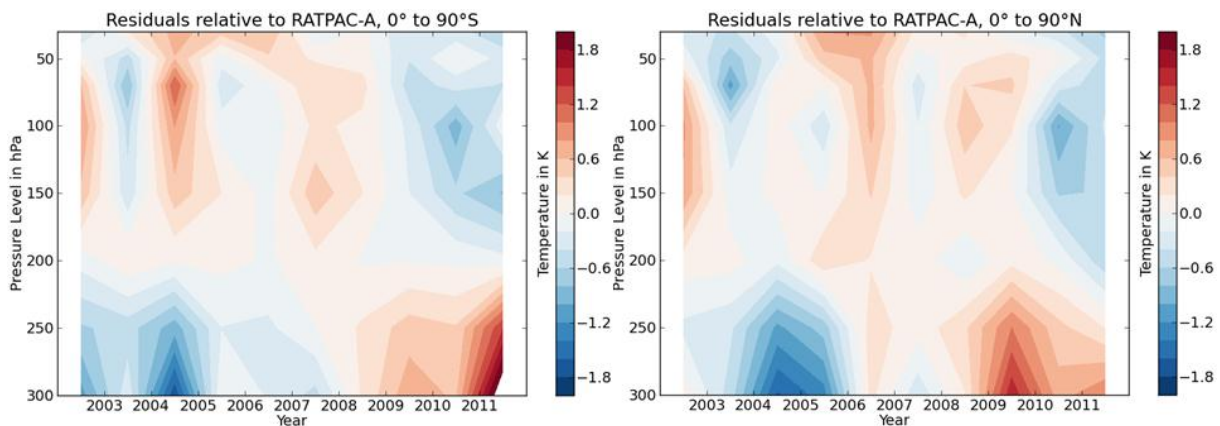
Figure 19: Differences between BSUTLS temperature anomalies and those from the RATPAC-A database. The leftmost panel shows differences for the southern hemisphere while the rightmost panel shows differences for the northern hemisphere.
