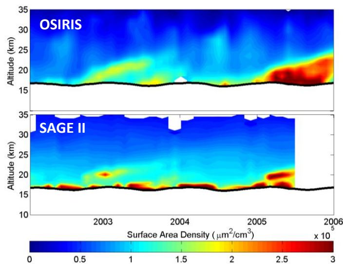
Figure 31: Monthly averaged surface area density from OSIRIS in the top panel and SAGE II in the bottom panel.
