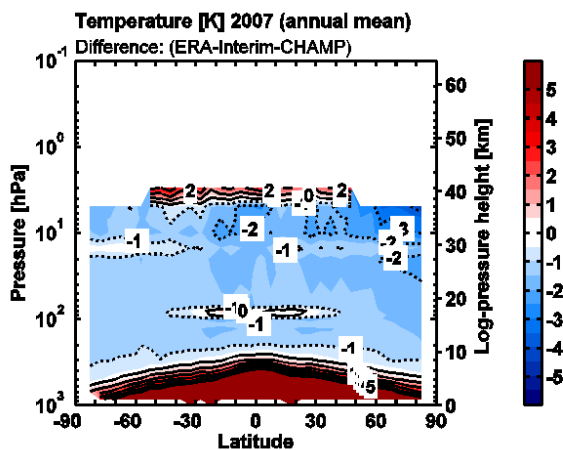
Figure 5: Annual mean temperature difference (ERA-Interim minus CHAMP) for 2007.
