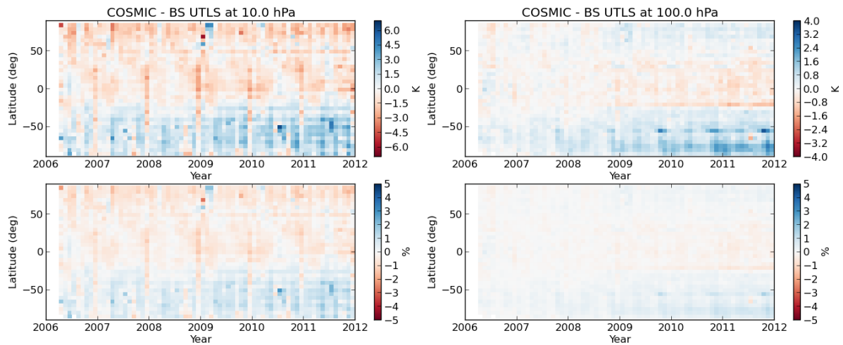
Figure 22: Differences between the BSUTLS and COSMIC RO data sets at 10 hPa (leftmost panels) and at 100 hPa (rightmost panels). Upper panels show the differences in absolute units (K) while the lower panels show the percentage differences.
