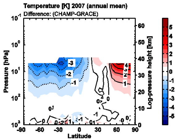
Figure 2: Annual mean temperature difference (CHAMP minus GRACE) for 2007.
