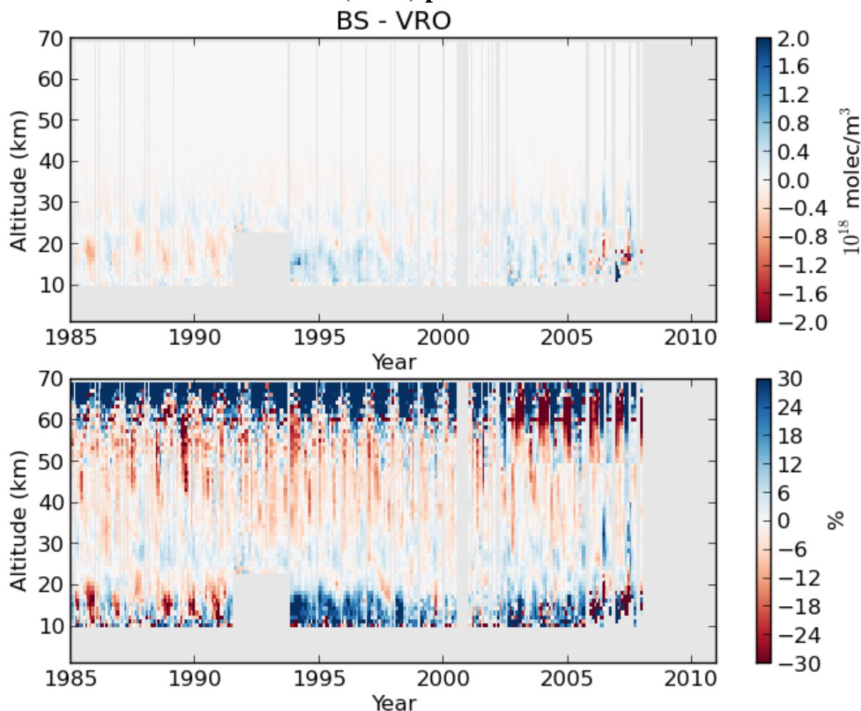
Figure 48: An example difference field between the Bodeker Scientific (BS) merged SAGE II and GOMOS ozone profile database and the Bodeker Scientific vertically resolved ozone database (VRO). The upper panel shows absolute differences in 10^{18} molec/m 3 while the lower panel shows the percentage differences. Greyed areas show where comparative data are not available. These results are for the region 40°S to 45°S.
