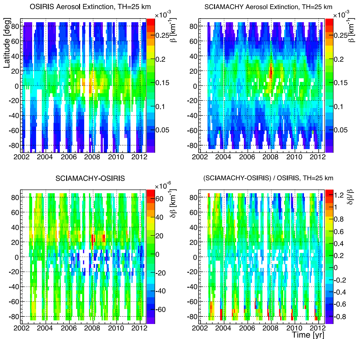
Figure 40: Top: OSIRIS (left) and SCIAMACHY (right) aerosol extinction at 25 km vs. latitude and time. Bottom: Absolute (left) and relative (right) differences of aerosol extinction (SCIA-OSIRIS) at 25 km vs. time.
