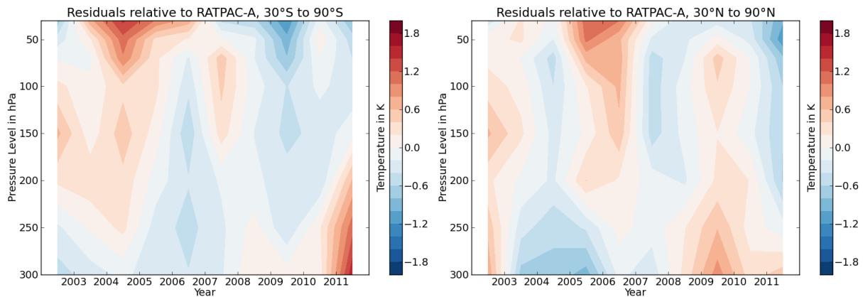
Figure 21: Differences between BSUTLS temperature anomalies and those from the RATPAC-A database in extra-tropics. The leftmost panel shows differences for the southern hemisphere while the rightmost panel shows differences for the northern hemisphere.
