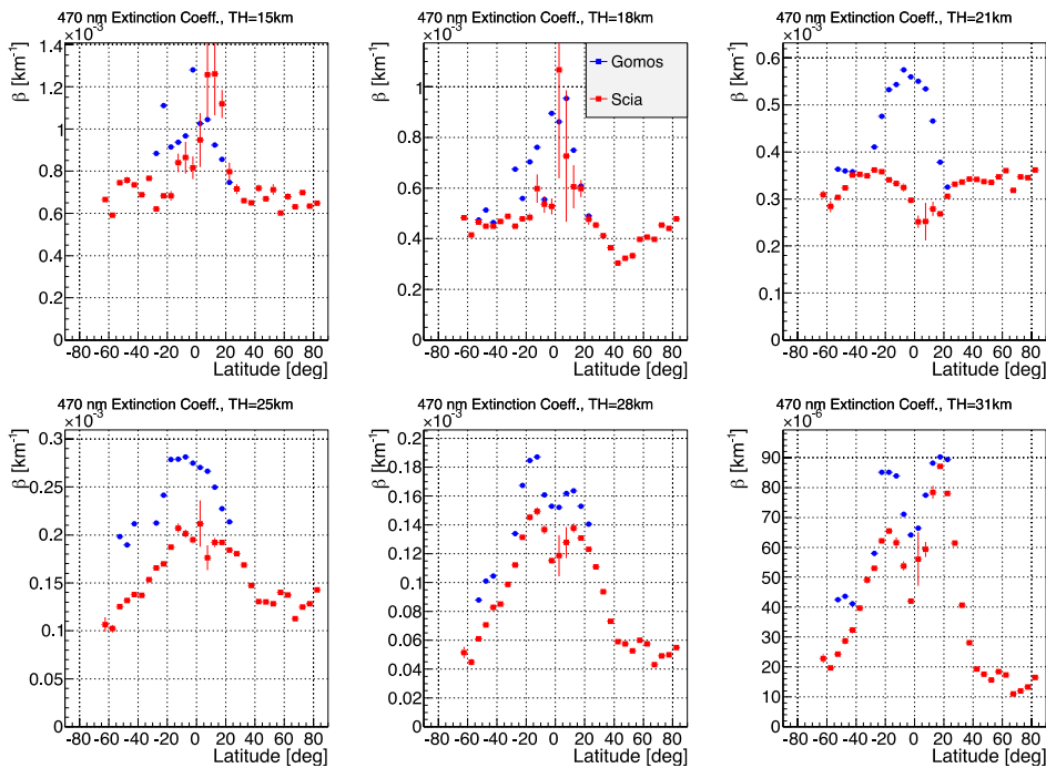
Figure 39: Monthly zonal mean aerosol extinction for June 2003 at 470 nm vs. latitude at 6 selected tangent heights, from SCIAMACHY and GOMOS.
