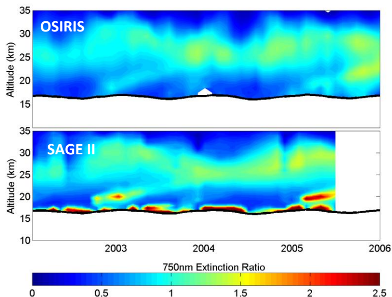
Figure 29: Monthly averaged 750 nm extinction ratio in the tropics. OSIRIS measurements shown in the top panel with SAGE II in the bottom panel.
