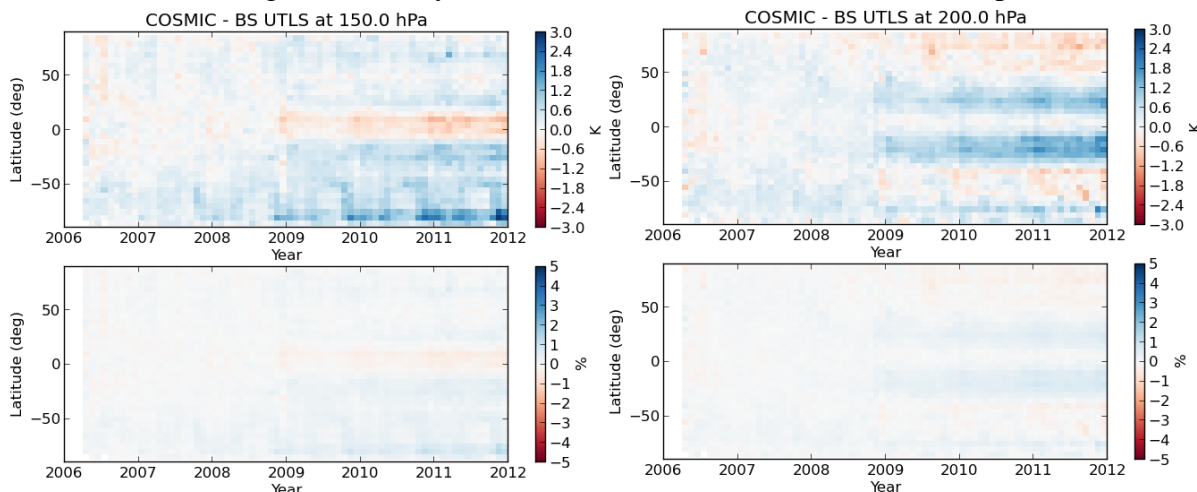
Figure 23: Differences between the BSUTLS and COSMIC RO data sets at 150 hPa (leftmost panels) and at 200 hPa (rightmost panels). Upper panels show the differences in absolute units (K) while the lower panels show the percentage differences.
