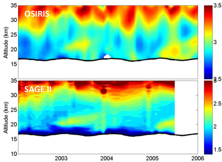
Figure 30: Top panel is the monthly OSIRIS Angstrom coefficient from 750 to 1530 nm from 20°N to 20°S. Bottom panel is the same picture with the SAGE II Angstrom coefficient from 525 to 1020 nm.
