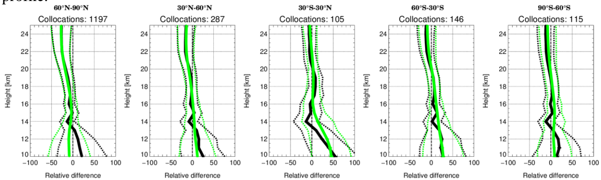
Figure 28: Comparison for SCIAMACHY V3.01 and ACE-FTS V3.0 for different latitude bands. Lines as in Figure 26.
