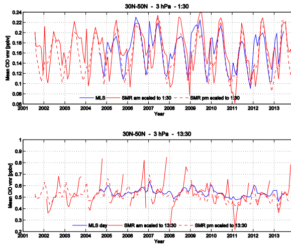
Figure 54: Comparison of local solar time scaled SMR (red) and unscaled MLS (blue) CIO time-series for the 3hPa level and northern mid-latitudes. Top: night (1:30am). Bottom: day (1:30pm).
