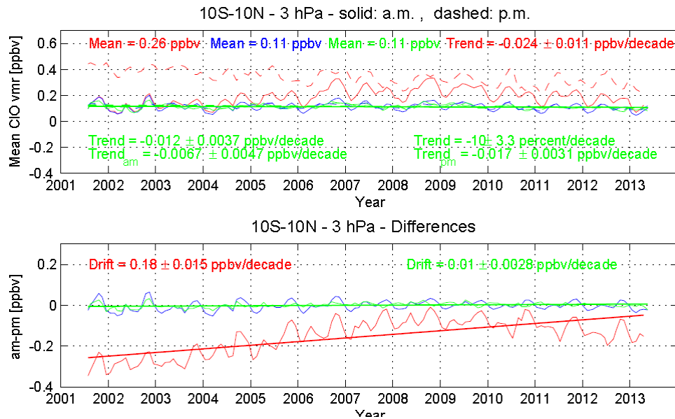
Figure 56: Internal consistency of CIO time-series based on measurements scaled to 1:30am at the 3hPa level in the tropics. Top: unscaled (red), scaled (blue), and deseasonalised scaled (green) time-series of morning (am: solid) and evening (pm: dashed) CIO observations by Odin/SMR. Bottom: Difference of am and pm scaled climatologies.
