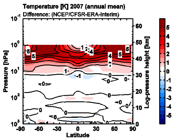
Figure 8: Annual mean temperature difference (NCEP-CFSR minus ERA-Interim) for 2007.
