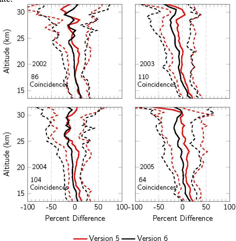
Figure 32: Comparison of SAGE III and OSIRIS aerosol retrievals for yearly coincident measurements. Mean per cent differences are shown as solid lines with standard deviation shown as dashed. Version 5.07 retrievals are shown in red with Version 6.00 shown in black.
