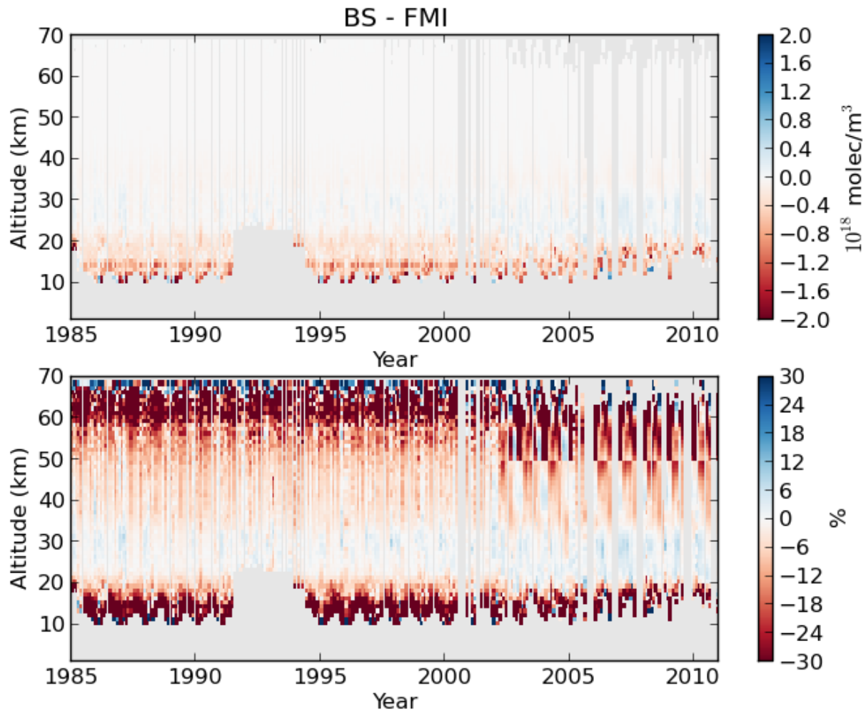
Figure 47: An example of the difference field between the Bodeker Scientific (BS) merged SAGE II and GOMOS ozone profile database and a similar database generated by FMI. The upper panel shows absolute differences in 10^{18} molecules/ m^3 while the lower panel shows the percentage differences. Greyed areas show where comparative data are not available. These results are for the region 30^{\circ}N to 40^{\circ}N .
