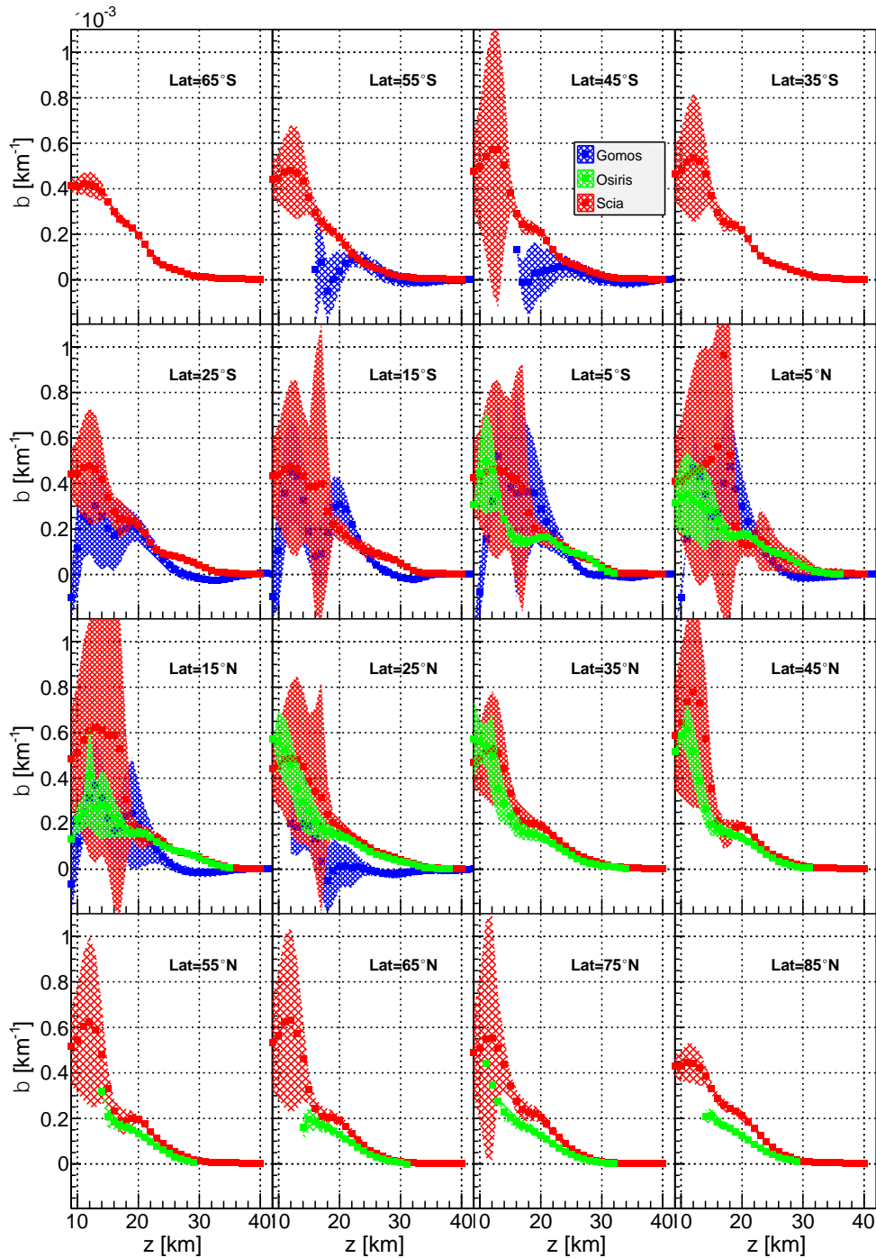
Figure 36: Monthly zonal mean aerosol extinction profiles at 750 nm from SCIAMACHY, GOMOS and OSIRIS for June 2003.
