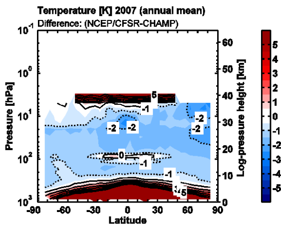
Figure 6: Annual mean temperature difference (NCEP-CFSR minus CHAMP) for 2007.
