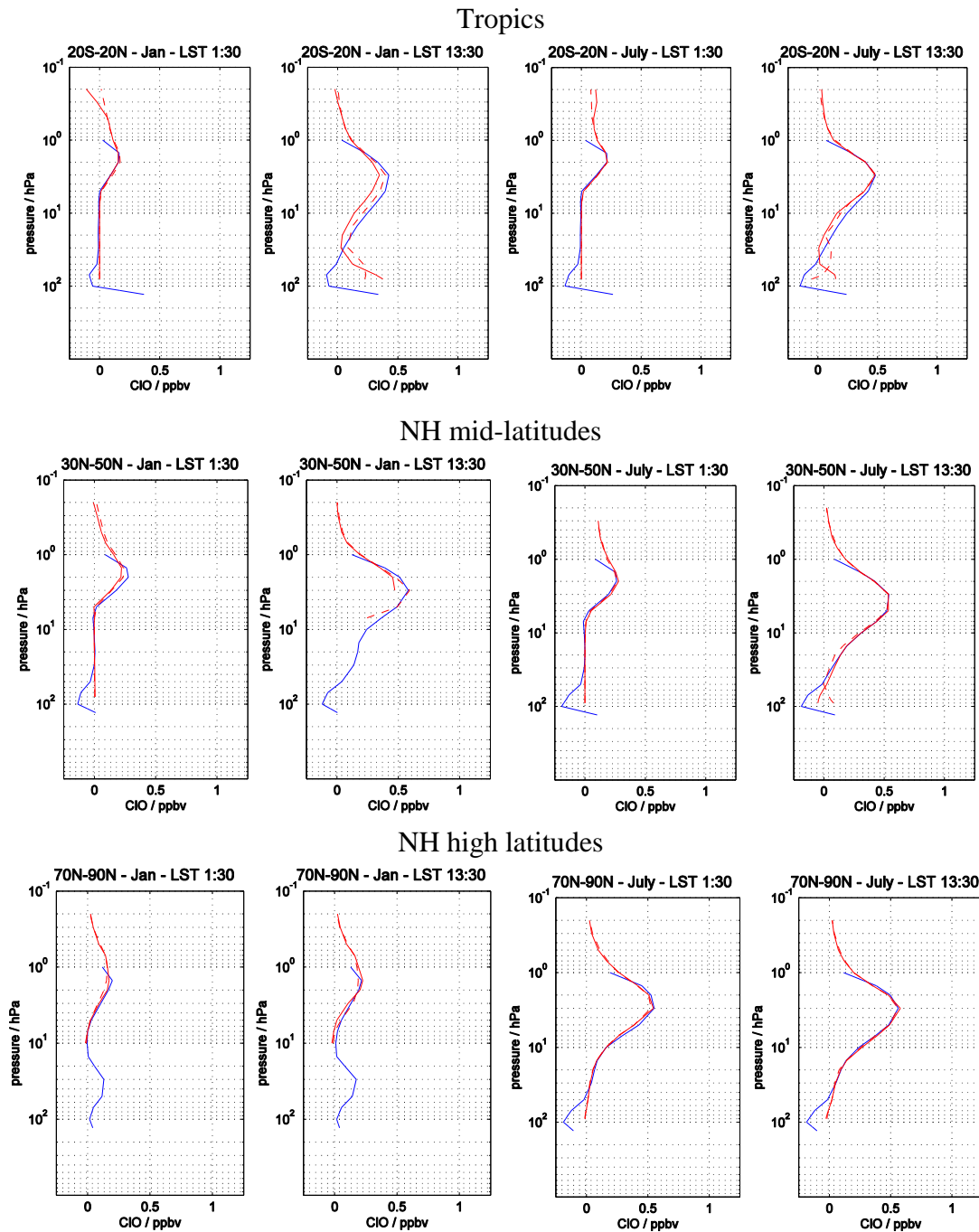
Figure 52: Comparison of local solar time scaled Odin/SMR climatological profiles (red) with unscaled MLS observations (blue) of ClO. Top: tropics; middle: northern mid-latitudes; bottom: northern high latitudes. Examples are shown for January (left) and July (right) and are averaged over the 2005-2012 period. For each month comparisons are shown for the two local times corresponding to day and night. Note that SMR climatologies are further distinguished into climatologies produced from am (morning: solid red line) and pm (evening: dashed red line) measurements.
