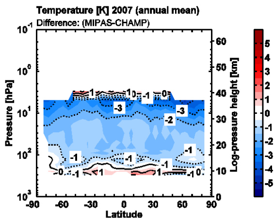
Figure 9: Annual mean temperature difference (MIPAS minus CHAMP) for 2007.
