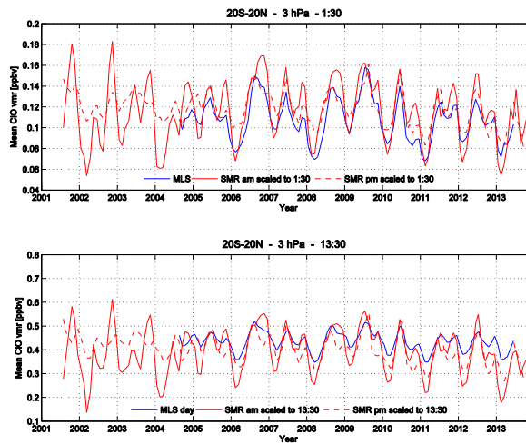
Figure 53: Comparison of local solar time scaled SMR (red) and unscaled MLS (blue) CIO time-series for the 3hPa level and the tropics. Top: night (1:30am). Bottom: day (1:30pm).
