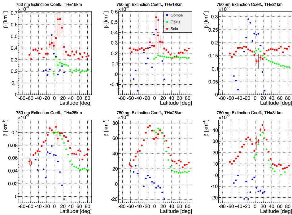
Figure 38: Monthly zonal mean aerosol extinction for June 2003 at 750 nm vs. latitude at 6 selected tangent heights, from SCIAMACHY, GOMOS and OSIRIS.
